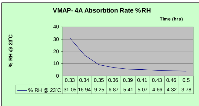
Graph 2 – Rate of Adsorption (% RH @ 23°C)
