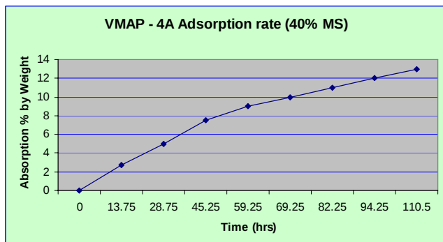
Graph 1 – Rate of Adsorption (% weight)
