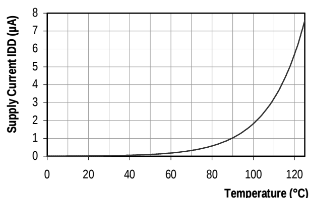
Figure 6 Typical dependency of supply current (sleep mode) versus temperature at VDD = 3.0V. Please note that the variance of these data is about \pm 25\% of displayed value.
