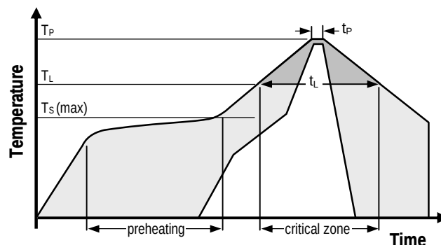
Figure 9 Soldering profile according to JEDEC standard. T_P \leq 260^\circ\text{C} and t_P < 40\text{sec} for Pb-free assembly. T_L < 220^\circ\text{C} and t_L < 150\text{sec} . Ramp-up/down speeds shall be < 5^\circ\text{C/sec} .
