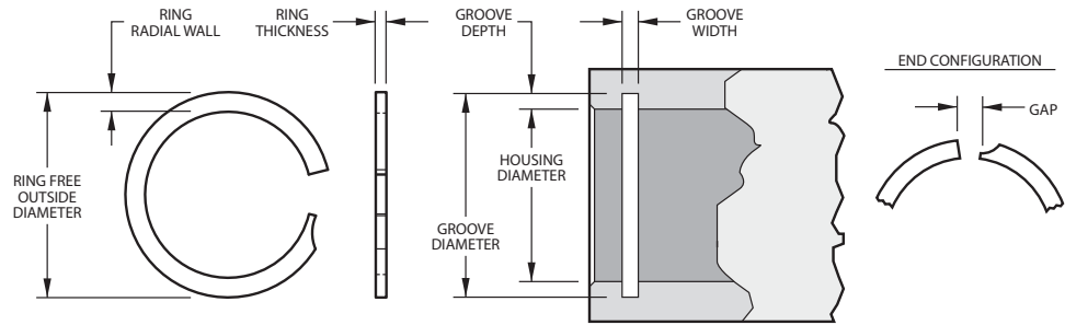
Product Dimensions All dimensions are in inches unless otherwise specified.
