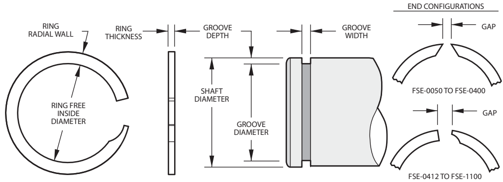
Product Dimensions All dimensions are in inches unless otherwise specified.
