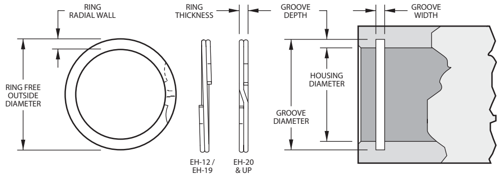
Product Dimensions All dimensions are in millimeters unless otherwise specified.
