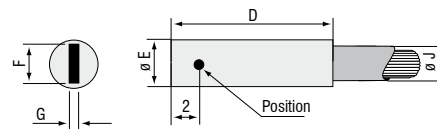
E Type E ferrule, stainless steel (* E1.0 only suitable for PVC sheathing)
