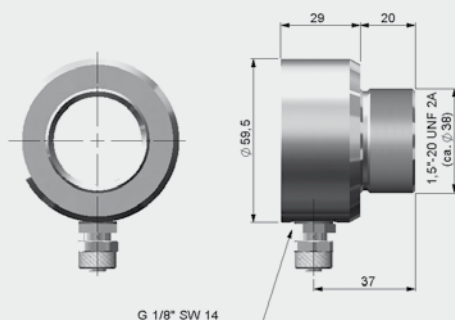
TM-AP-CX Air purge collar CX sensors
