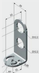
TM-FB2-CT Laser-Sighting mounting bracket
