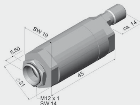
TM-AP2-CT Standard air purge collar for 2:1 optics
