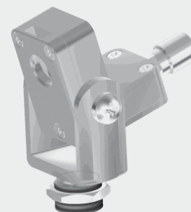
TM-APL-CS Laminar air purge collar and TM-MG-CS Mounting fork
