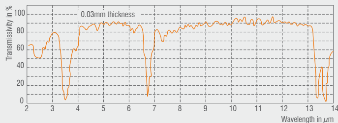
Spectral permeability of plastics made from poethylene.
