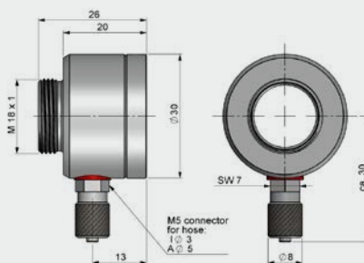
TM-APMH-CT Air purge collar, stainless steel for massive housing
