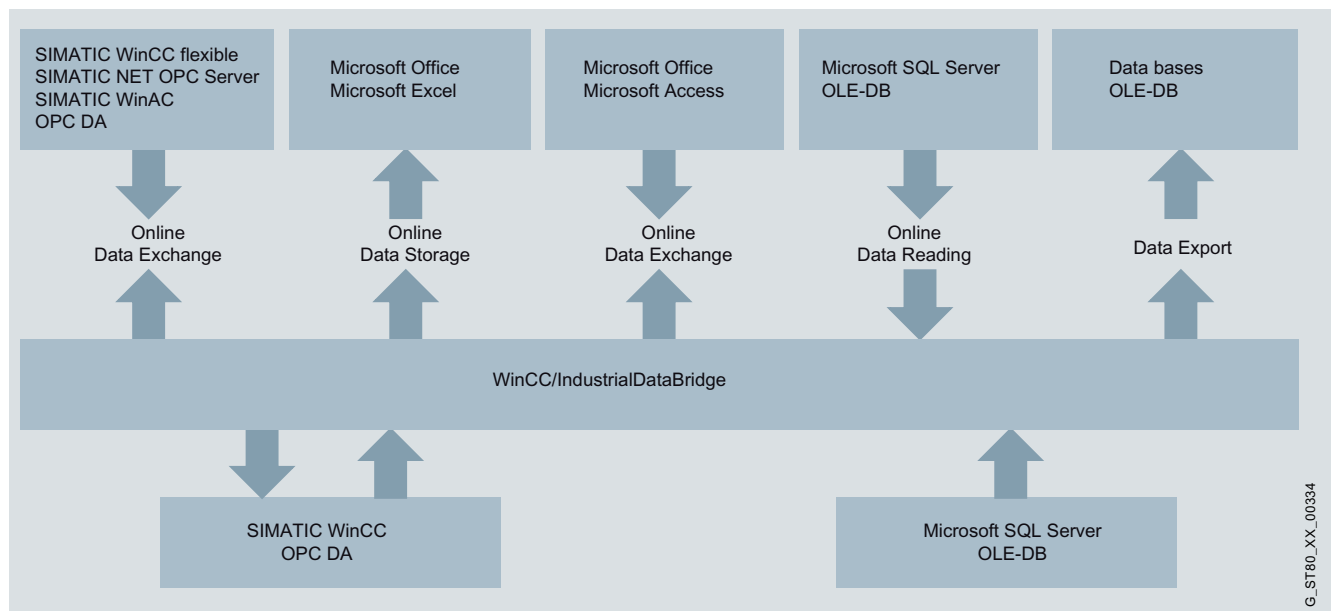
WinCC/IndustrialDataBridge: Connection to databases and IT systems
