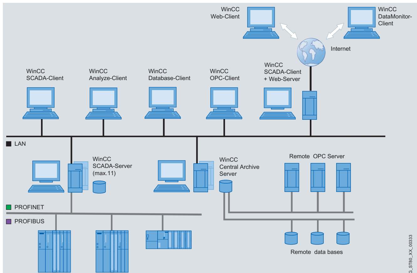
WinCC SCADA Client as web server for different clients in the web with central process data archiving
