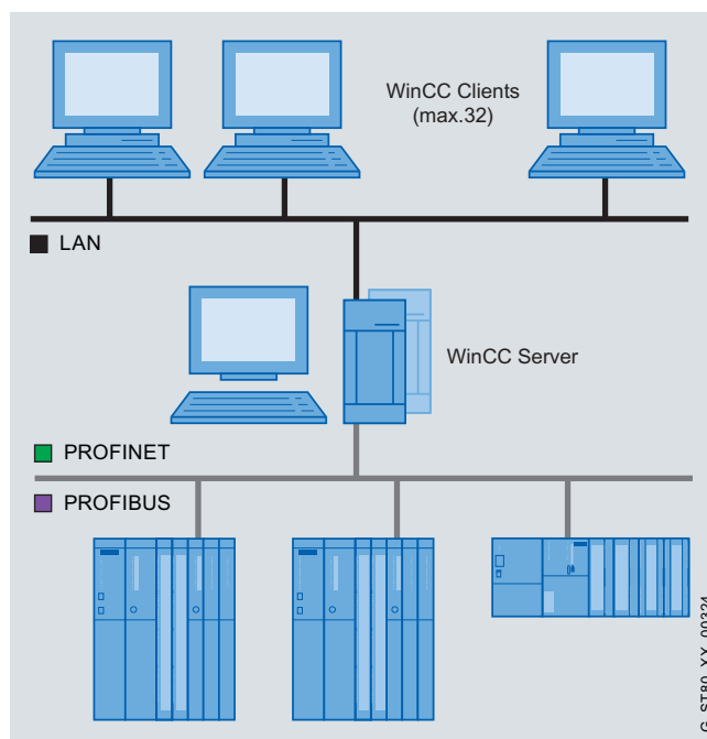
WinCC multi-user system
