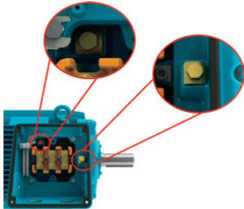
Figure 7 - Earth terminals in the terminal box
