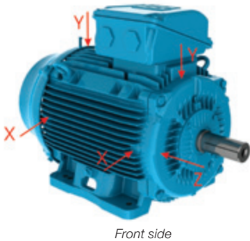
Figure 6 - Flat surfaces for vibration monitoring on the back and front side
