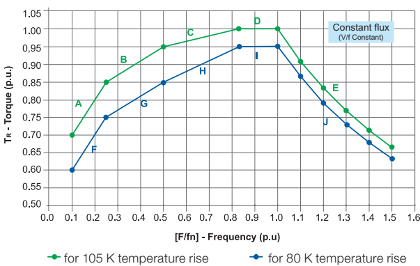
Figure 32 - Derating curves for constant flux condition
